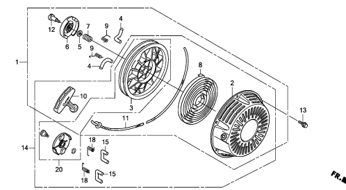
RECOIL STARTER(1)
